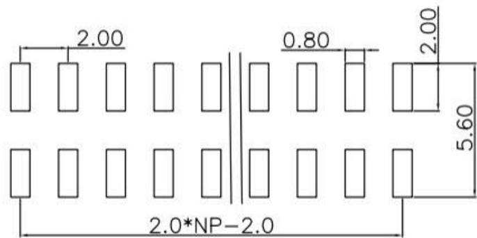
PCB LAYOUT
