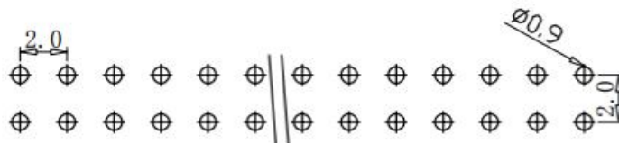
PCB LAYOUT
