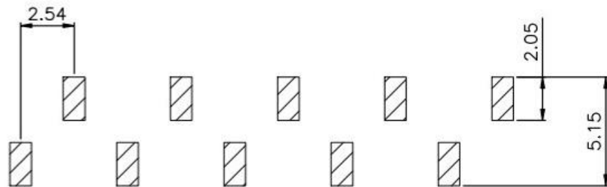
PCB LAYOUT
