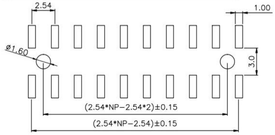
PCB LAYOUT
