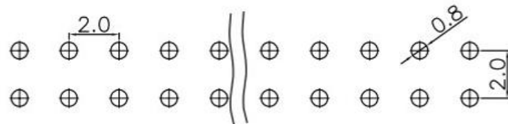
PCB LAYOUT
