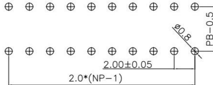
PCB LAYOUT
