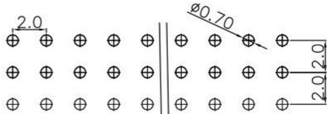
PCB LAYOUT
