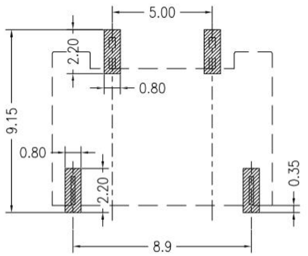
Board Layout
