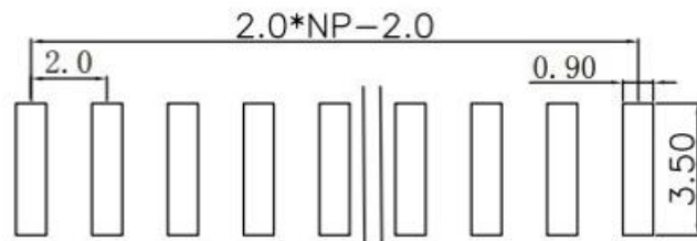
PCB LAYOUT
