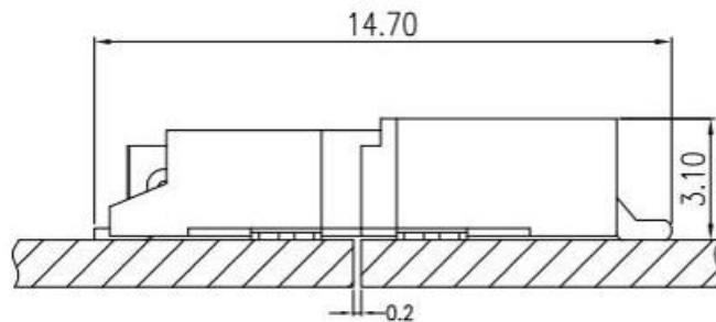
Assembly Layout
