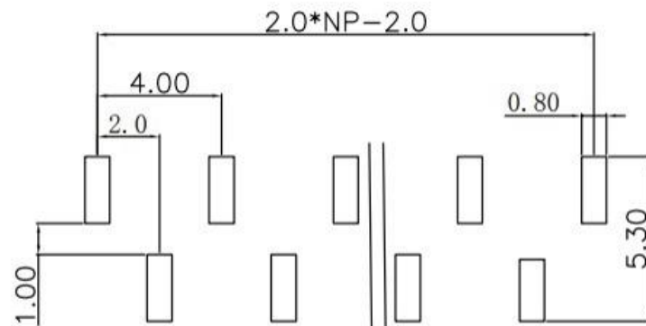
PCB LAYOUT
