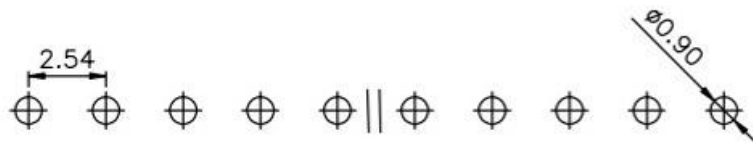
PCB LAYOUT
