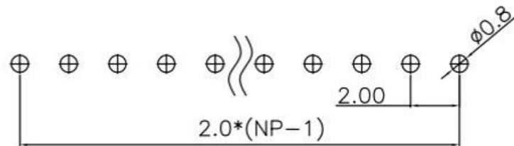
PCB LAYOUT
