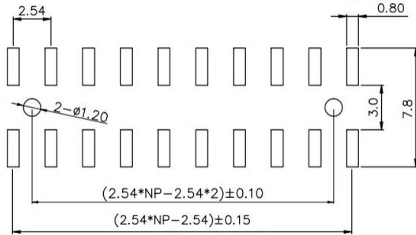
PCB LAYOUT
