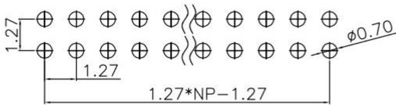
PCB LAYOUT
