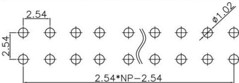
PCB LAYOUT
