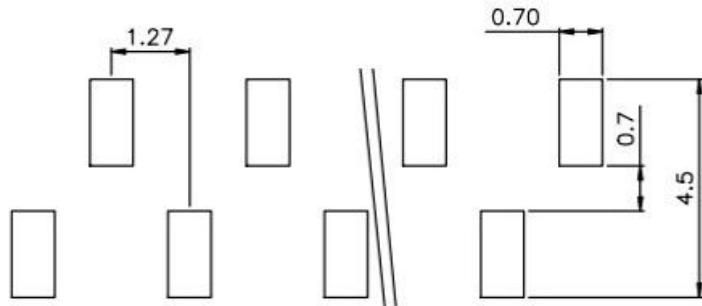
PCB LAYOUT
