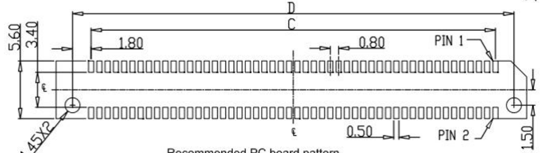
Recommended PC board pattern (TOP VIEW)
