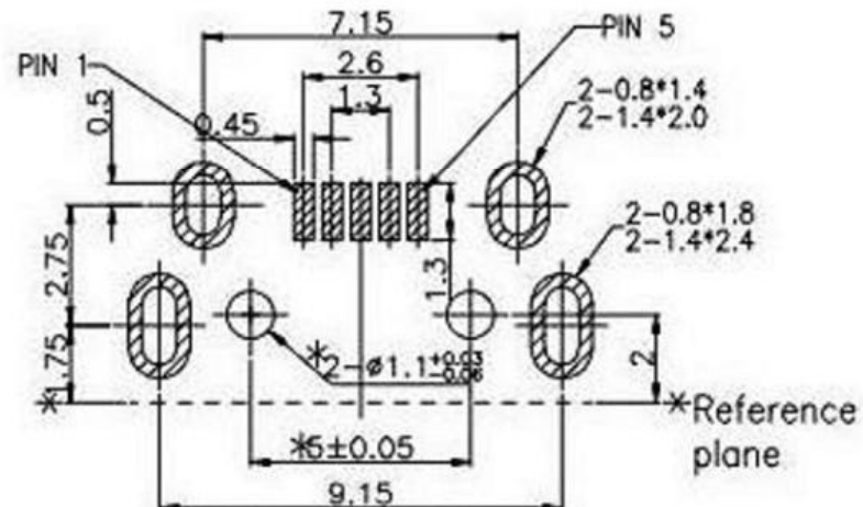
Recommended PCB Layout Tolerance: ±0.1(Top view)
