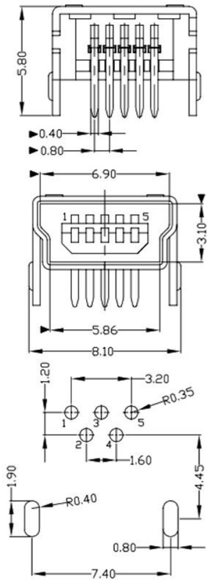
RECOMMENDED PCB LAYOUT
