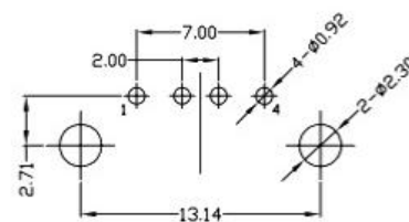
RECOMMEND PCB LAYOUT
