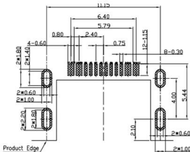
RECOMMENDED P.C.B. LAYOUT TOLERANCE UNSPECIFIED ±0.05mm
