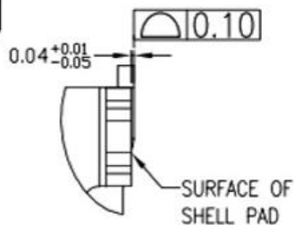
DETAIL B (2:1)
