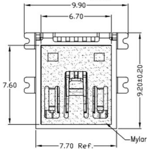
DETAIL B (2:1)
