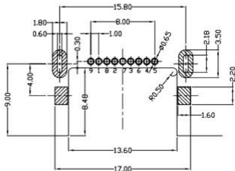
RECOMMENDED PCB LAYOUT(1.0~1.60±0.05)
