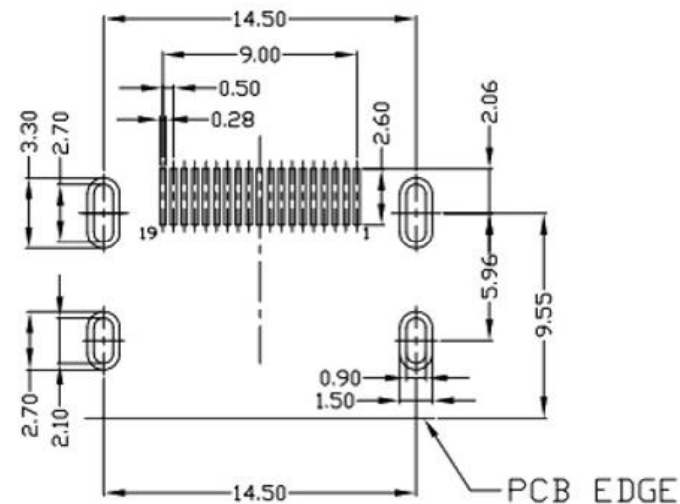
RECOMMENDED PCB LAYOUT (T=1.60mm)
