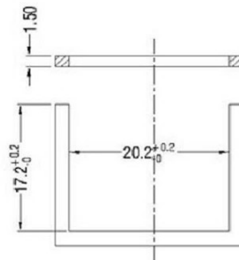
PANLE CUT-OUT
