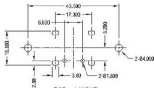
PCB LAYOUT THICKNESS: 1.6mm
