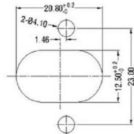
PANEL CUT-OUT
