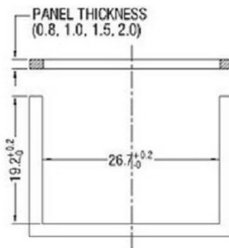
PANEL CUT-OUT
