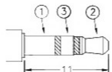
2.5mm MATE PLUG
