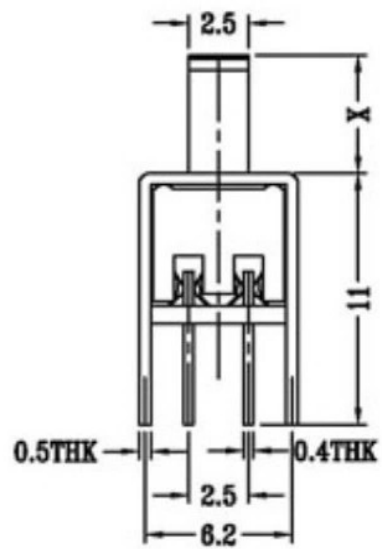
SCHEMATIC (SHORTING)
