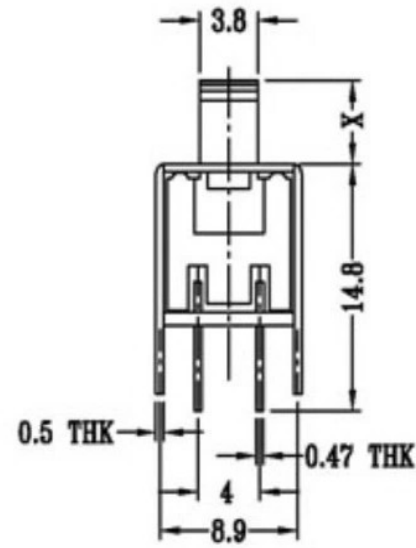
SCHEMATIC (SHORTING)
