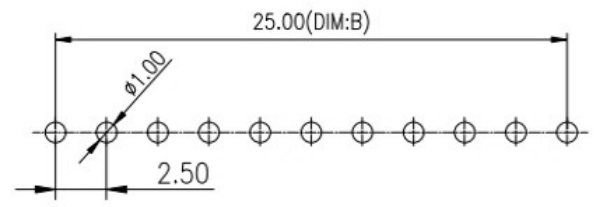
Recommended P.C.B Layout Layout Tolerance=+/-0.05mm
