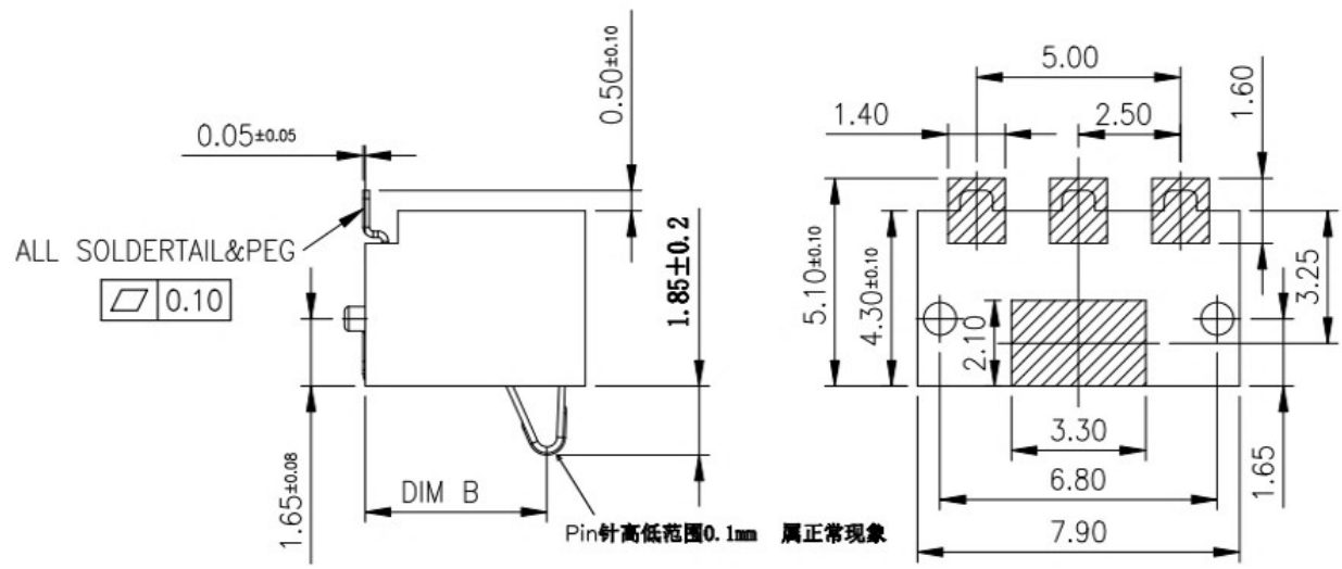
RECOMMENDED PCB LAYOUT TOP VIEW (.XX±0.05)
