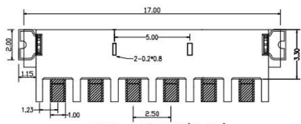
PCB LAYOUT(6pin)
