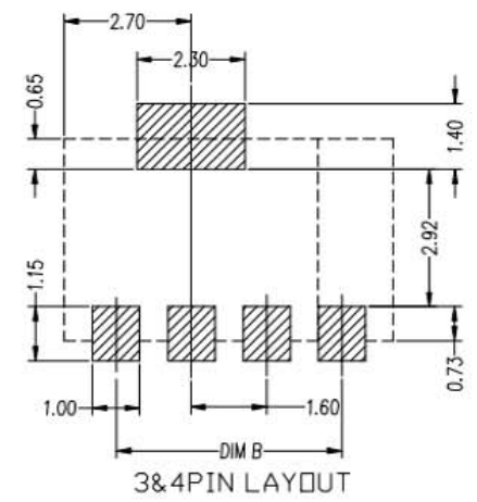
3&4PIN LAYOUT RECOMMENDED PCB LAYOUT TOL:(±0.05)
