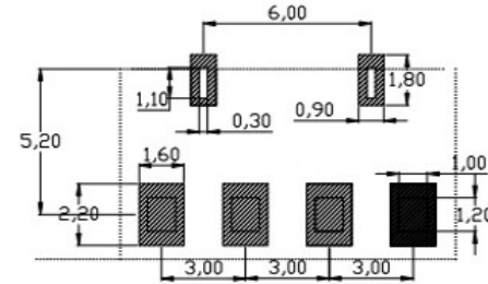
RECOMMENDED PCB LAYOUT TOP VIEW (. XX±0.05)
