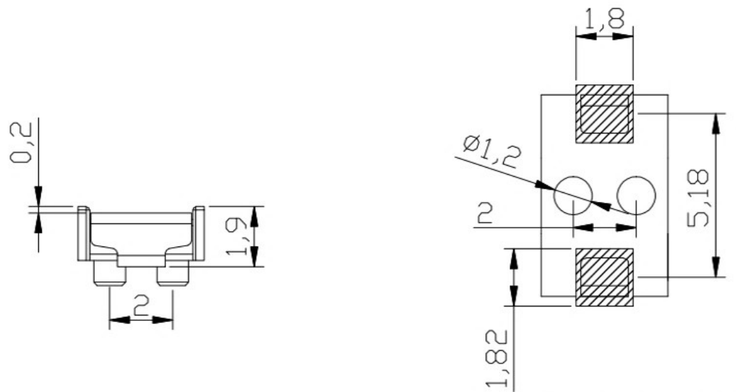
RECOMMENDED PCB LAYOUT TOP VIEW(. XX±0.05)
