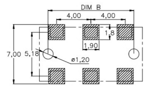
RECOMMENDED PCB LAYOUT TOP VIEW (.XX±0.05)
